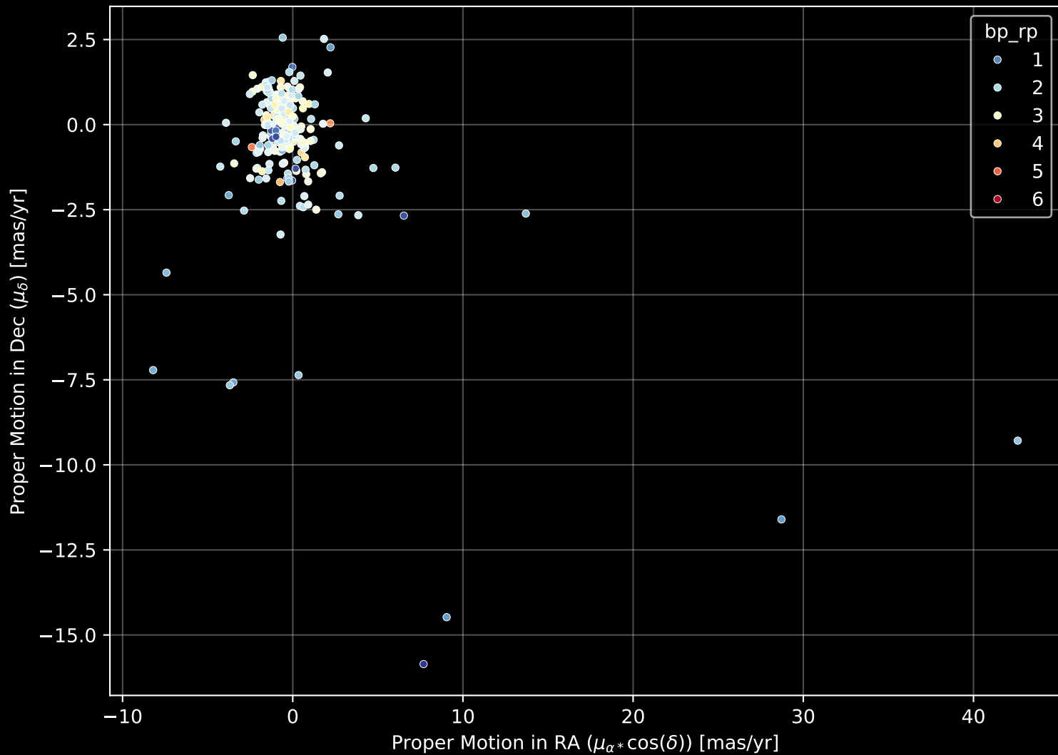
APOGEE DR17 Field: [131+00] Proper Motion Diagram (n= 250)
