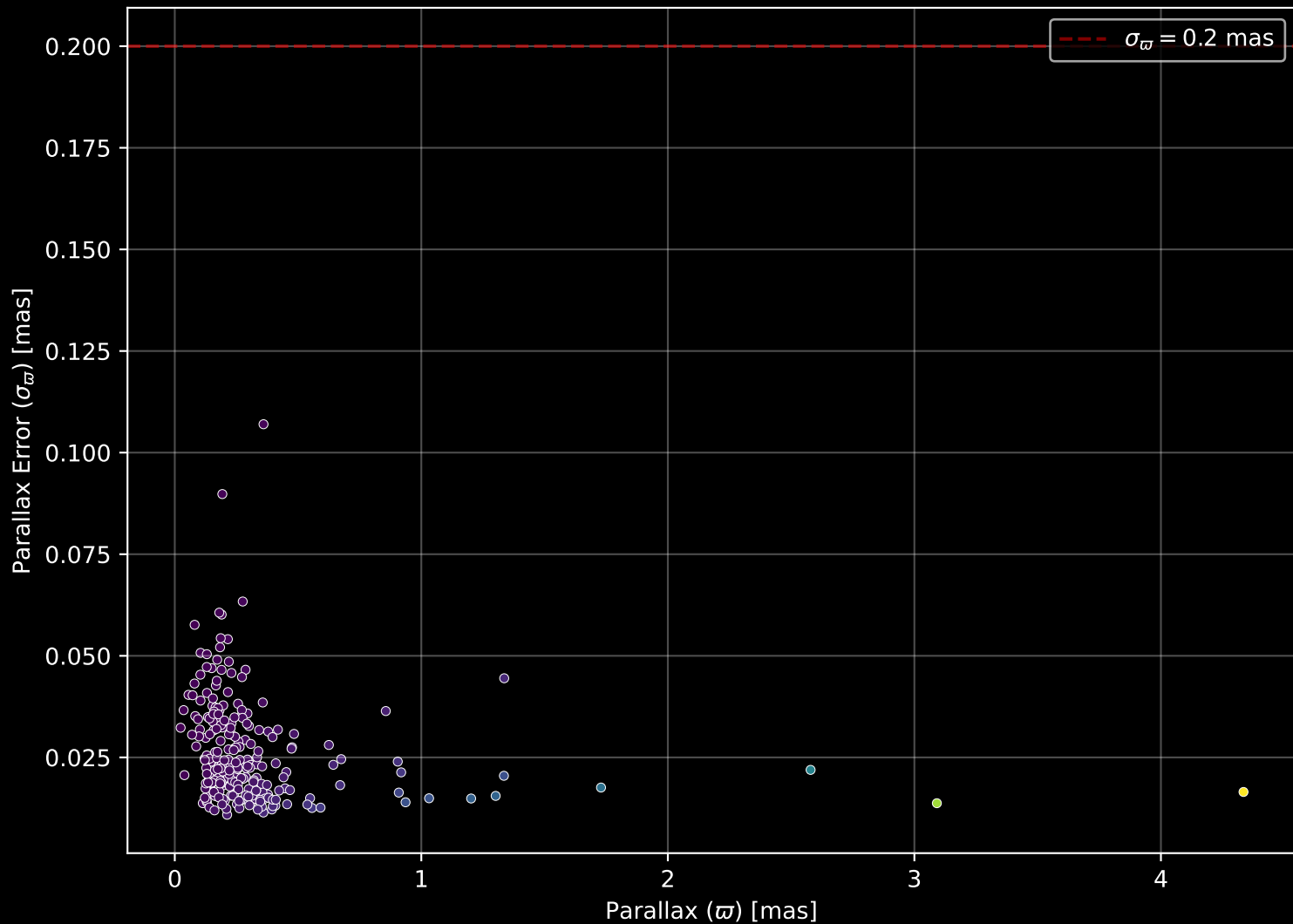
APOGEE DR17 Field: [131+00] Parallax Quality (n= 250)
