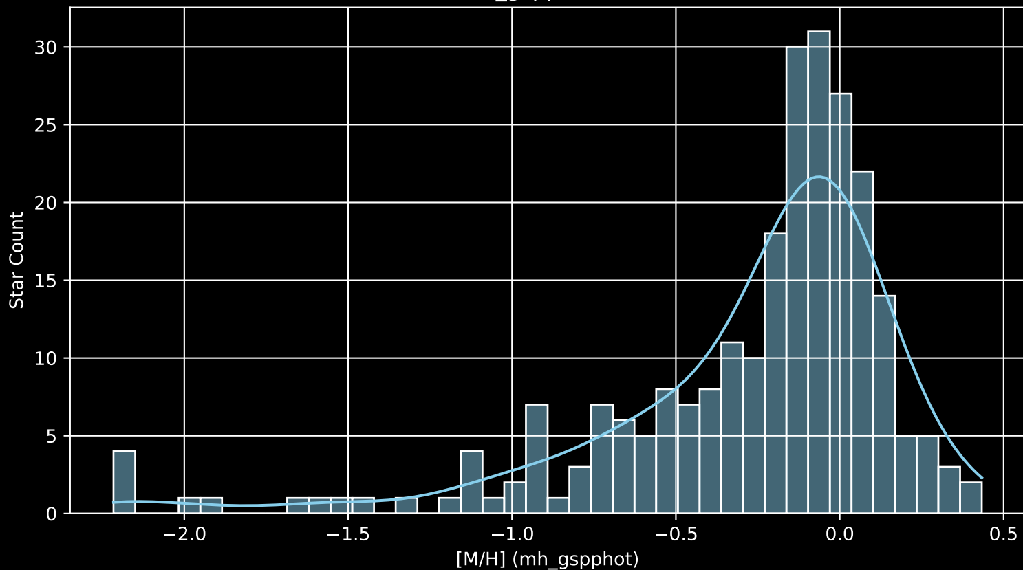
APOGEE DR17 Field: [131+00 [M/H] (mh_gspphot) (n= 249)
