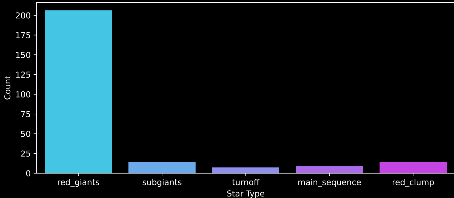
APOGEE DR17 Field: [131+00] Count plot of Star Type
