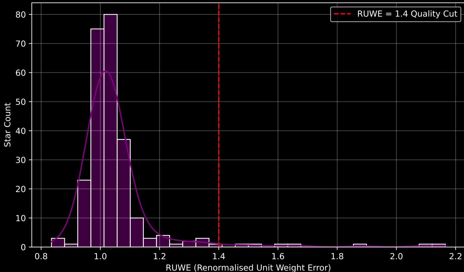
GAPOGEE DR17 Field [131+00] RUWE Distribution (n= 250)
