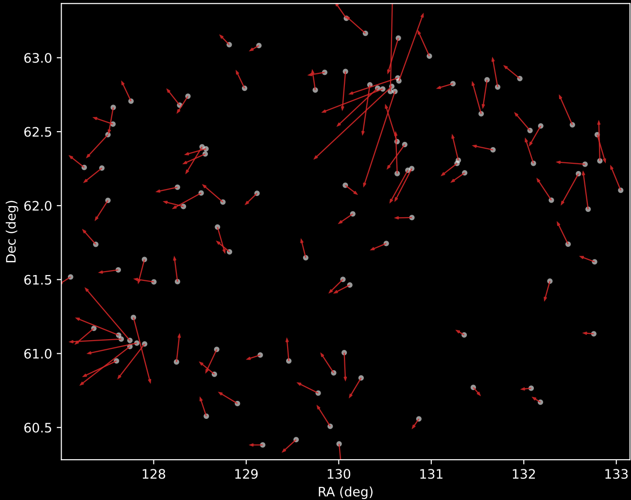
APOGEE DR17 Cluster 6 Proper Motion Vectors (n=108)
